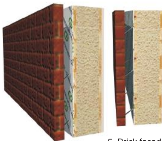
5. Brick facade (with ties - 6 pcs./m 2 )
