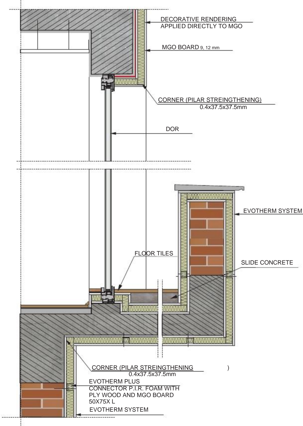
VERTICAL SECTION
